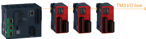
Modicon M262 Logic/Motion controller controlling TM3 functional safety modules: local I/O connected to the TM3 I/O bus
